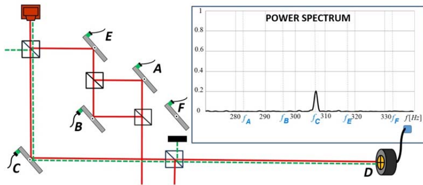
FIG. 1D: The forward and backward evolving states are present together only at mirror C and thus, the only peak in the power spectrum is at f_C . Since according to the naïve approach the presence of peaks at f_A and f_B in Figure 1B is very counterintuitive, one might suspect that these peaks may result from some unrelated electronic noise. A block between mirror F and the last beam splitter absorbs the backward evolving wave moving towards mirrors F , A , B , and E . In the language of the forward wave function only, it absorbs the leakage of the wave from the inner interferometer. Thus theoretically, according to the standard and the TSVF approaches, the block ensures the absence of peaks at the corresponding frequencies. Therefore, this experiment provides a decisive test for the absence of electronic noise in Figure 1B.
