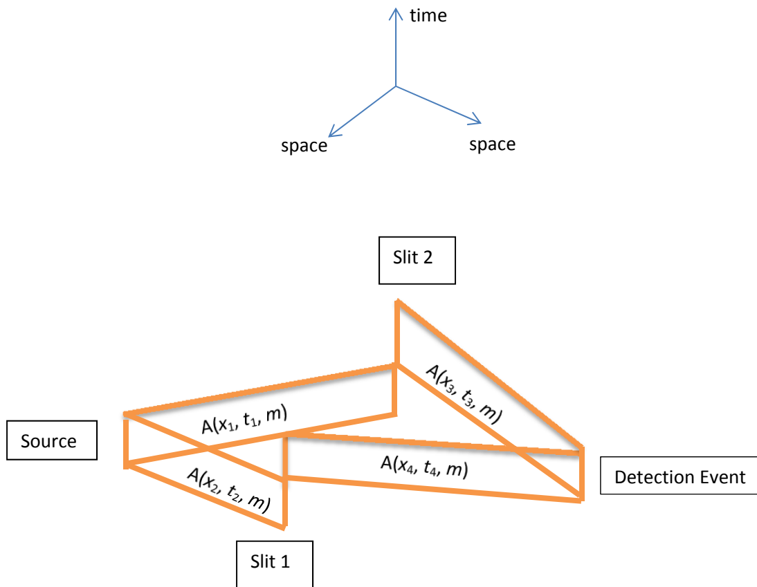
Fig 7. The boxes are the components of the spacetimesource element depicting mass m loss at the Source emission event and mass m gain at the Detection Event contributing to an interference pattern at the detector.
